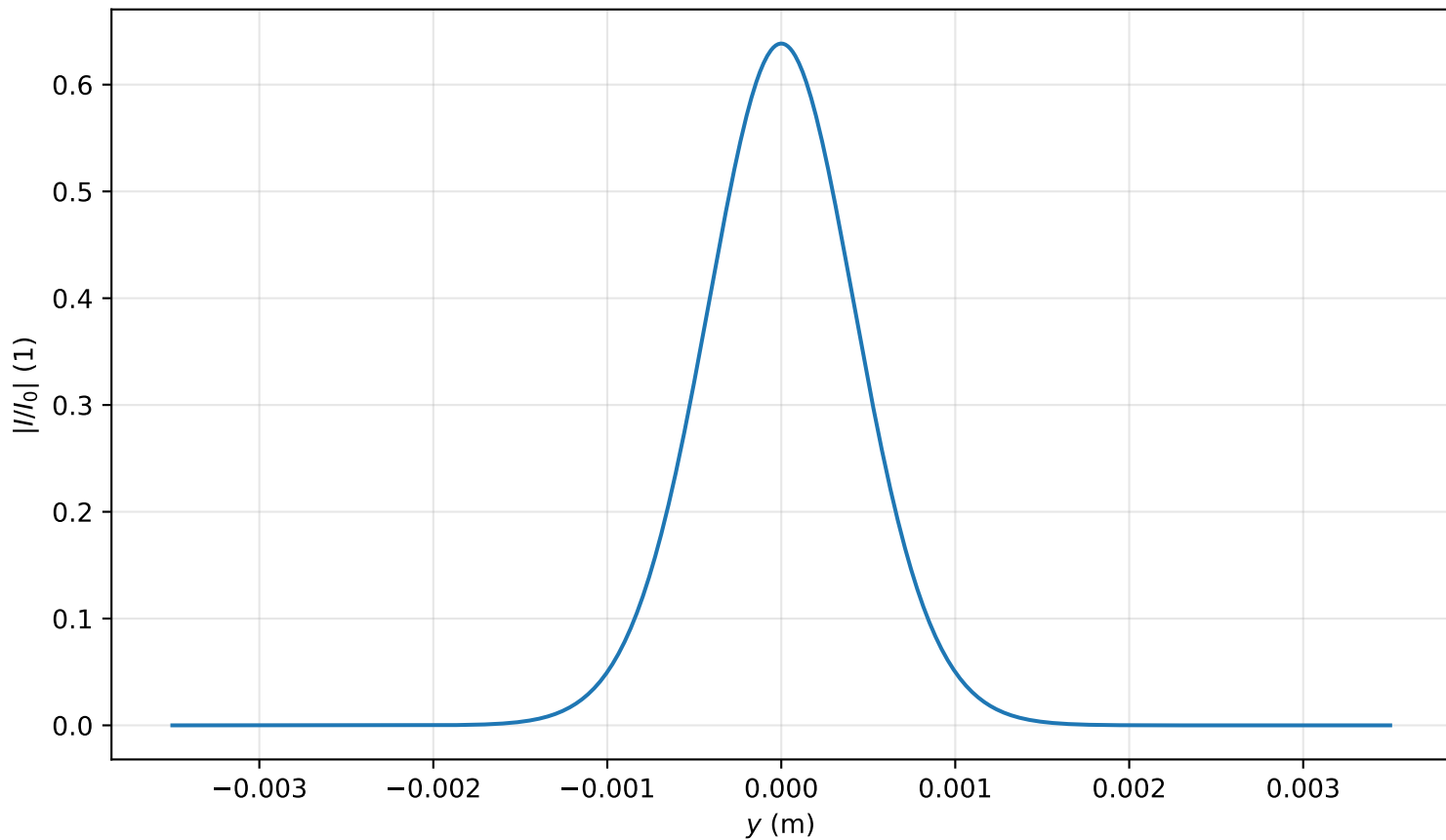
Intensity profile I(x=0, y, z=1.831)/I_0 , P_{in}=0.2P_{cr} , artificial time
